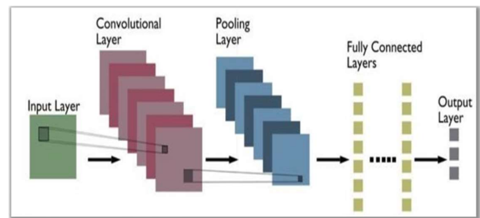
Fig.7 CNN Architecture
